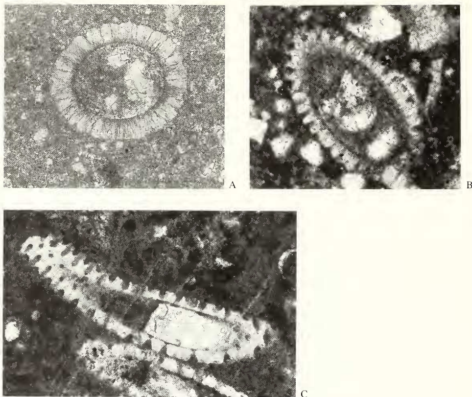
TEXT-FIG. 1. A–C, Hensonella dinarica (Radoičić). A, WG23; Early Aptian, Shuaiba Formation; Oman; transverse section showing inner micritic wall and radial calcitic structure, \times 80 . B, WM105; Hauterivian–Barremian, Kharaiib Formation; Oman; transverse section showing radial structure and dasycladacean verticils, \times 80 . C, RR019440/A309; Barremian–Aptian; Zeta Plain, Yugoslavia; oblique transverse section of a toptype of Salpingoporella dinarica Radoičić, showing dasycladacean verticils and faint radial calcitic structure, \times 60 . Specimens WG23 and WM105 are held in the Biostratigraphy Reference Collection, BP Research Centre, Sunbury-on-Thames, UK; specimen RR018440/A309 is held in the collection of Petroconsultants, Geneva, Switzerland.
